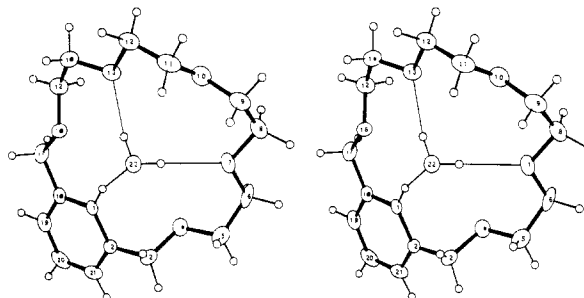
Figure 2. Stereoscopic view of the 2,6-pyridino-18-crown-6-H 2 O-HClO 4 (1:1:1) complex (5), showing atom numbering. The perchlorate ion is omitted.
